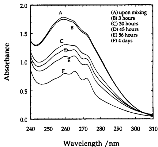
Figure 4. Changes in the UV spectrum of 1.8 \times 10^{-4} \text{ M} \text{PPh}_3 and 1.0 \times 10^{-4} \text{ M} \text{CH}_3\text{ReO}_3 over a period of 4 days in 1:1 \text{CH}_3\text{CN}-\text{H}_2\text{O} at pH 1.0.
