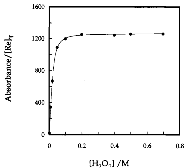
Figure 3. Plot of the absorbance at 360 nm of \text{CH}_3\text{ReO}_3-\text{H}_2\text{O}_2 solutions as a function of [\text{H}_2\text{O}_2] at [\text{Re}]_{\text{T}} = 1.0 \text{ mM} . The fit to eq 6 yields K_1 = 14 \pm 2 \text{ M}^{-1} and K_2 = 128 \pm 22 \text{ M}^{-1} . Conditions: pH 1.0 in 1:1 \text{CH}_3\text{CN}-\text{H}_2\text{O} at 25.0 °C.
