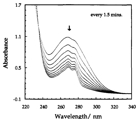
Figure 2. Repetitive spectral changes at 1.5-min intervals for the oxidation of 1.0 \times 10^{-4} \text{ M} (p\text{-CF}_3\text{C}_6\text{H}_4)_3\text{P} with 3.0 \times 10^{-3} \text{ M} \text{H}_2\text{O}_2 in the presence of 2.0 \times 10^{-6} \text{ M} \text{CH}_3\text{ReO}_3 at pH 1.0 in 1:1 \text{CH}_3\text{CN}-\text{H}_2\text{O} .
