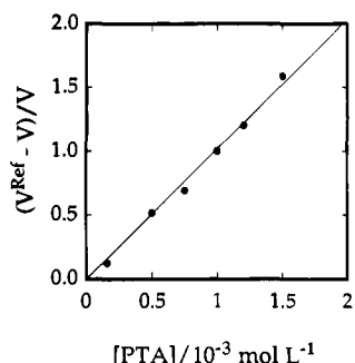
Figure 11. The rate-enhancement function, [v_p(\text{P}(\text{C}_6\text{F}_5)_3) - v_s(\text{PTA})]/v_s(\text{PTA}) , varies linearly with [\text{PTA}] according to eq 11 for competition experiments. Conditions: 25.0 °C, pH 1.0, 2.5 \times 10^{-4} M \text{P}(\text{C}_6\text{F}_5)_3 , 3.0 \times 10^{-4} M \text{CH}_3\text{ReO}_3 , 1.0 \times 10^{-4} M \text{H}_2\text{O}_2 .
